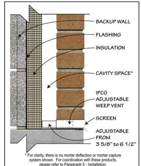
ADJUSTABLE VERTICAL WEEP FOR HEAD JOINTS
