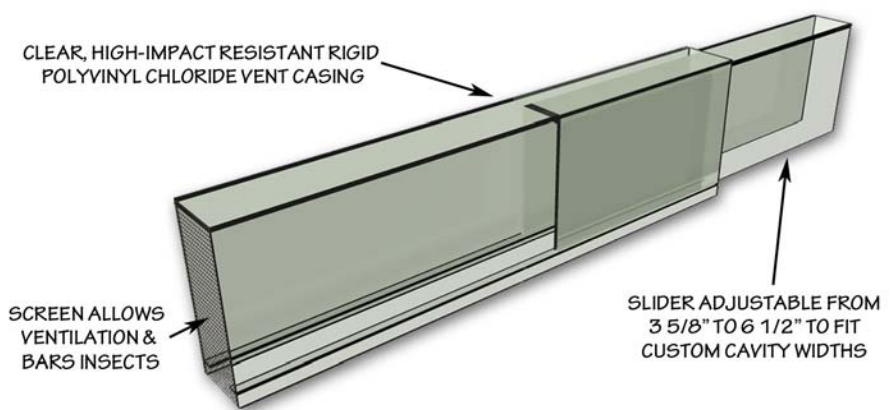
ADJUSTABLE VERTICAL WEEP FOR HEAD JOINTS
